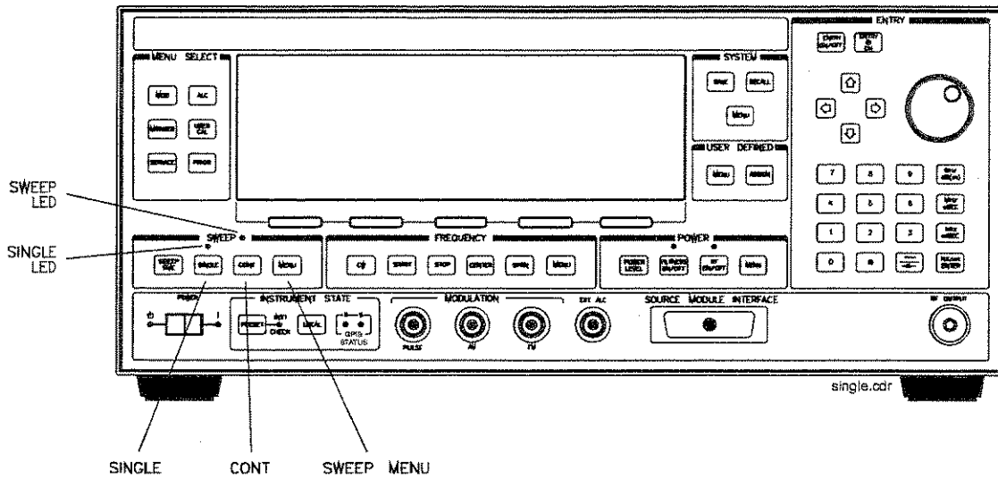
Figure 1-7. Continuous, Single, and Manual Sweep Operation
