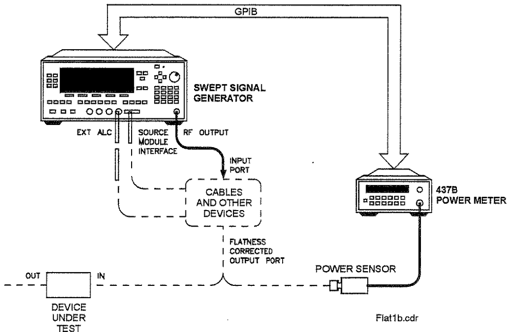
Figure F-1. Basic User Flatness Configuration Using an HP/Agilent 437B Power Meter
