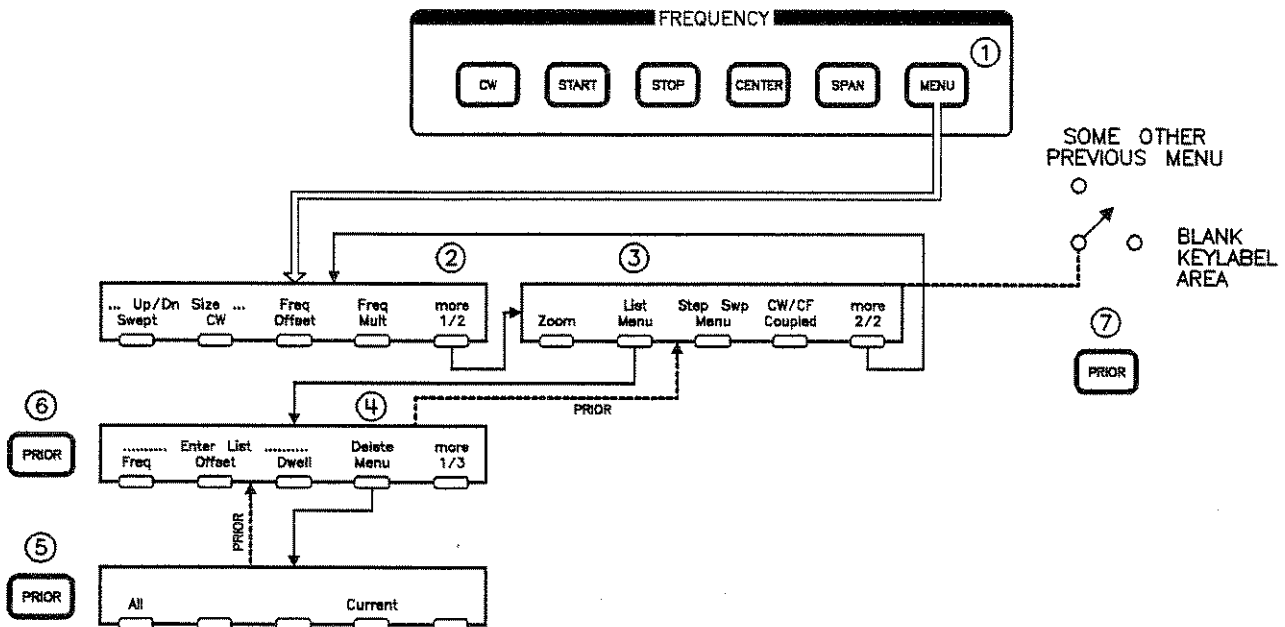
Figure P-1. How PRIOR Works
