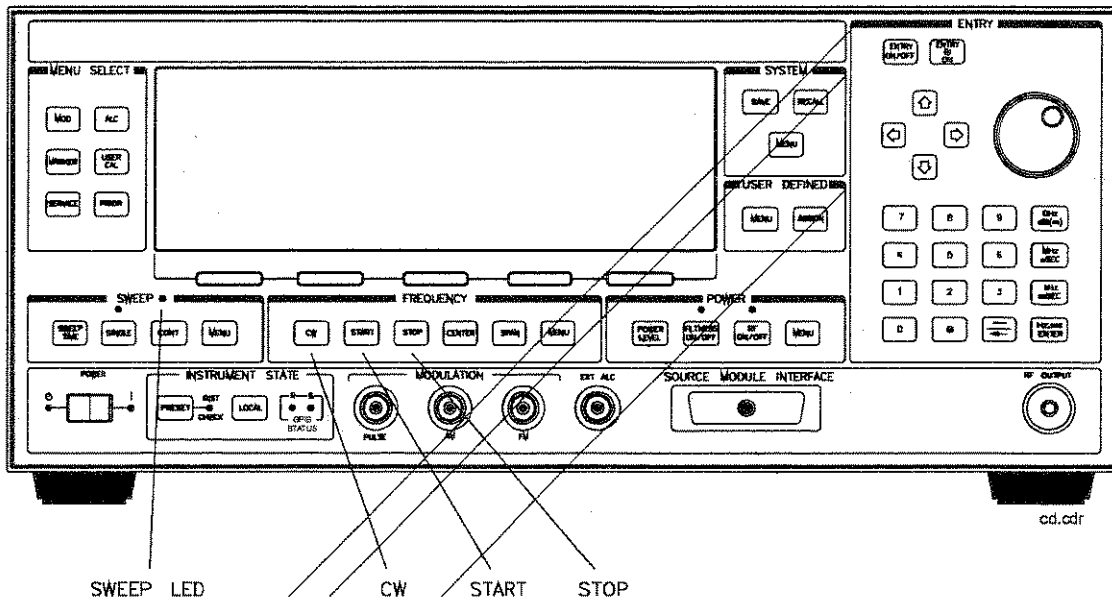
Figure 1-4. CW Operation and Start/Stop Frequency Sweep
