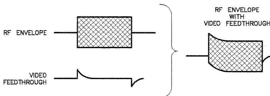
Figure M-6. Video Feedthrough
