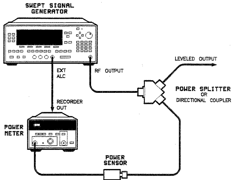
Figure 1-13. Leveling with a Power Meter
