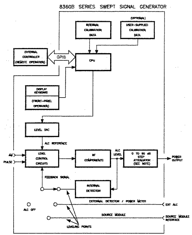
Figure A-1. ALC System Simplified Block Diagram
